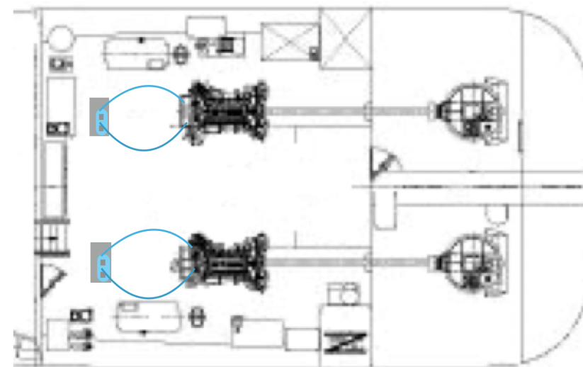
Ruang Mesin Tugboat
