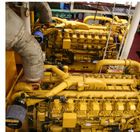
Mesin Tugboat
